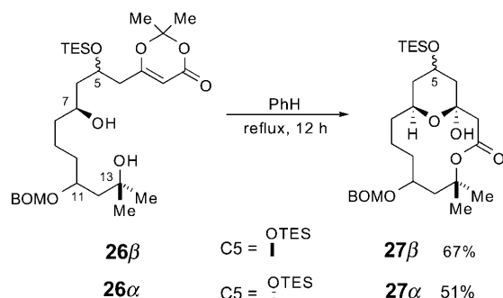
Scheme 4. Dual macrolactonization/pyran-hemiketal formation of substrates relevant to the synthesis of lynghyaloside B ( 6 ). Each of 26 \beta , 26 \alpha , 27 \beta , and 27 \alpha was an approximate 1:1 mixture of C11 epimers. TES = triethylsilyl, BOM = benzyloxymethyl.
